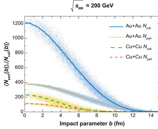
Figure 1.9: The average number of binary collisions, \langle N_{coll} \rangle , and that of participant nucleons, \langle N_{part} \rangle , as a function of the impact parameter b . The event-by-event fluctuations are added as the scatter plot. The Woods-Saxon distribution with R_A = 6.38 fm and a = 0.535 for ^{197}\text{Au} and R_A = 4.20641 fm and a = 0.5977 fm for ^{63}\text{Cu} are assumed, respectively. The measured \sigma_{inel}^{NN} = 42 mb is used in this calculation [50].
