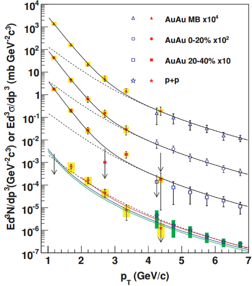
Figure 1.20: Invariant cross section (p+p) and invariant yield (Au+Au) of direct photons as a function of p_T . The filled points are obtained by the virtual photon analysis and open points are from [96, 97]. The three curves on the p+p data represent NLO pQCD calculations, and the dashed curves show a modified power-law fit to the p+p data, scaled by T_{AA} . The dashed (black) curves are exponential plus the T_{AA} scaled p+p fit.
