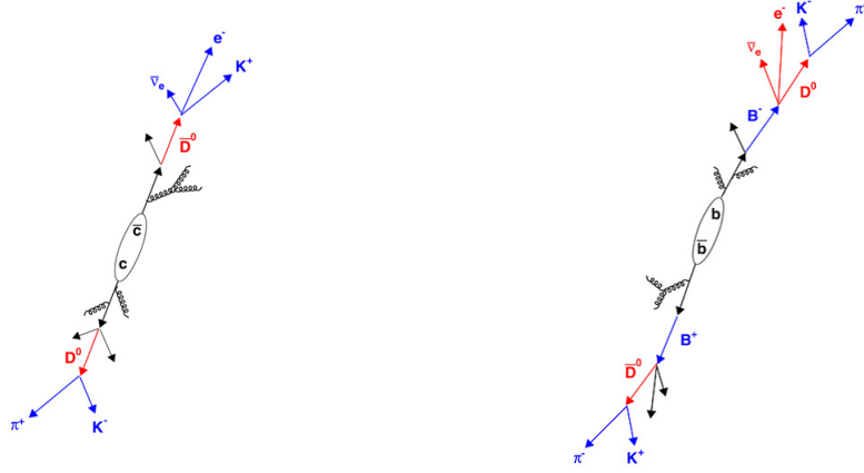
Figure 2.2: Semi-leptonic decay from charm and bottom [152].
