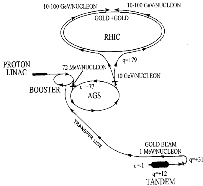
Figure 3.1: The overview of the RHIC complex and acceleration scheme for heavy ions.
