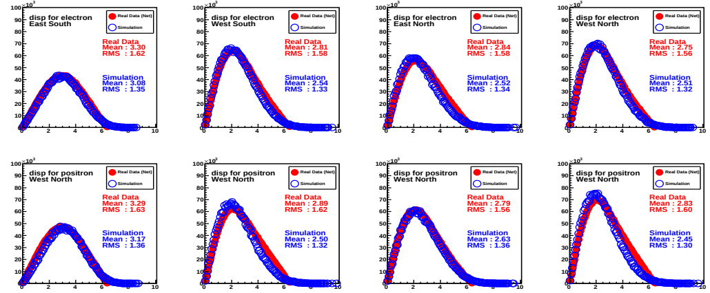
Figure 4.16: The comparison of the net distribution between the real data and the simulation, taking the RICH misalignment effect into account. The comparisons are shown for East-South, West-South, East-North and West-North. The top and bottom plots are disp distribution for electrons and positrons, respectively.
