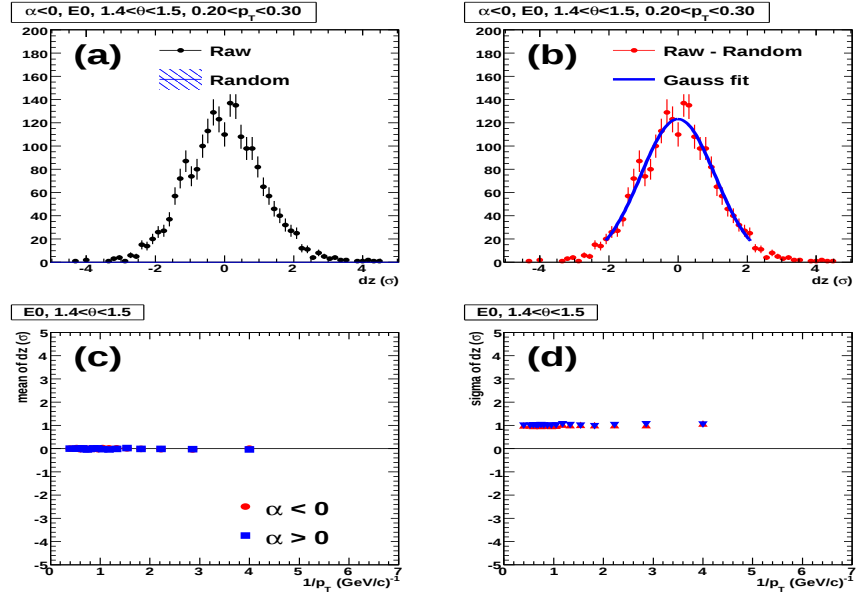
Figure 4.23: The normalized track matching parameter emcsdz_e of the simulation after the calibration.
