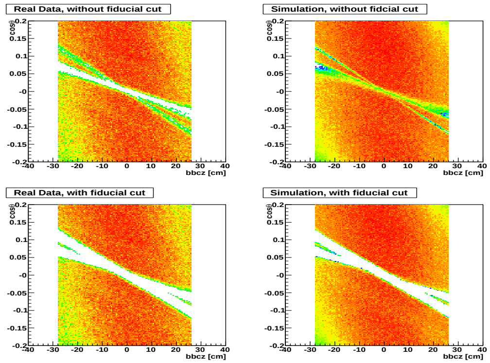
Figure 4.30: \cos\theta vs \text{bbc}z .
