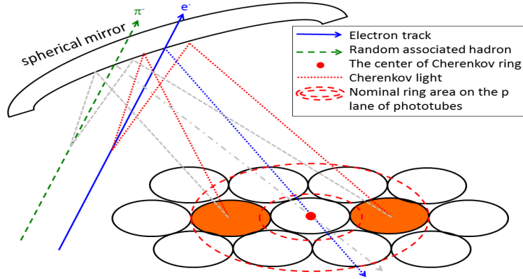
Figure 4.35: Schematic diagram of the ring sharing effect in RICH.
