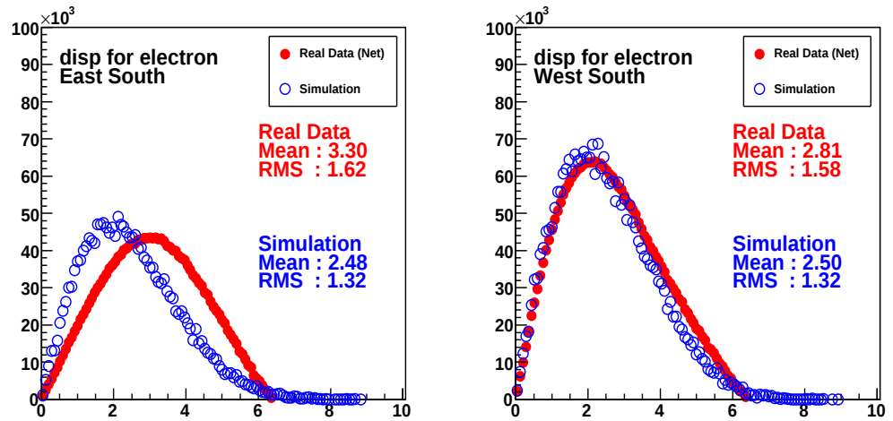
Figure 4.13: disp distribution of the east-south sector (left) and the west-south (left).
