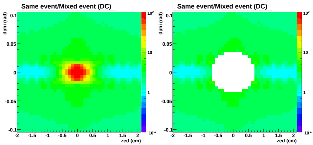
Figure 4.38: The relative amplitude of the pairs in the parameter space (dz_{\text{ed}}, d\phi) . The left and right plots show the relative amplitude before and after rejecting ghost tracks, respectively.
