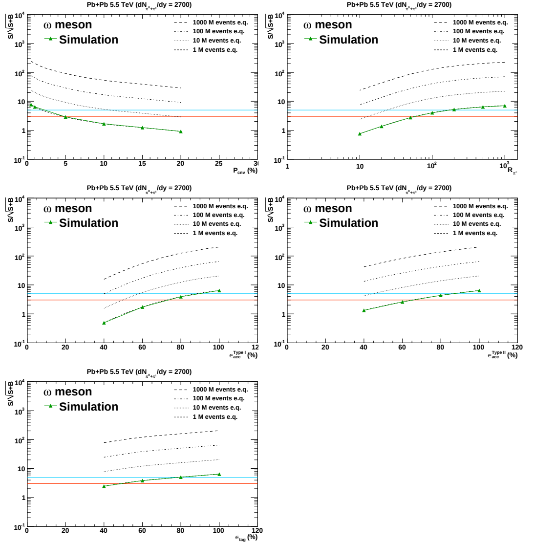
Figure 7.6: The statistical significance S/\sqrt{S+B} of \omega mesons as a function of the experimental parameters P_{cnv} , R_{\pi^\pm} , \epsilon_{acc} and \epsilon_{tag} in central Pb+Pb collisions at \sqrt{s_{NN}} = 5.5 TeV ( dN_{\pi^0+\pi^\pm}/dy = 2700 ). Only one parameter is changed by fixing the other parameters at the baseline values for each plot. The results of the simulation are shown as the symbols and the empirical curves are superimposed on the data points as the solid curves. The other dotted curves are the scaled curves with the square root of the expected number of events found in the highest centrality class. Two horizontal lines indicate S/\sqrt{S+B} = 3 and 5.
