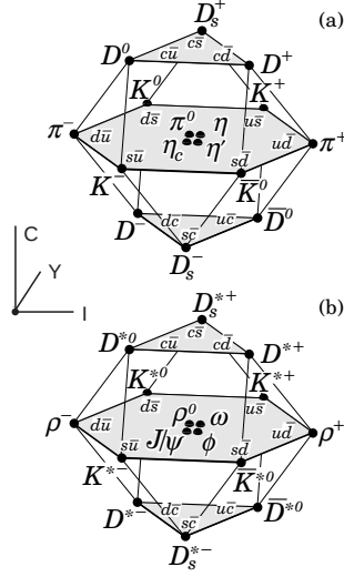
Figure 1.2: SU(4) multiplets (a 15-plet + singlet) for the pseudoscalar mesons (a) and the vector mesons (b) made of u , d , s and c quarks as a function of isospin I , charm C and the hyper charge Y = S + \mathcal{B} - C/3 . The nonets of light mesons occupy the central places to which the c\bar{c} states have been added.
