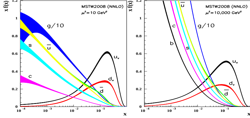
Figure 1.6: The unpolarized parton distribution times x for u_v, d_v, \bar{u}, \bar{d}, s, c, b and g at a factorization scale of \mu^2 = 10 \text{ GeV}^2 (left) and 10000 \text{ GeV}^2 (right).
