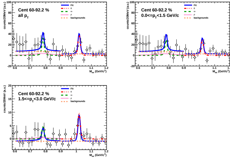
Figure 4.53: The invariant mass spectra of the di-electrons after subtracting event mixing distribution at the centrality class of 60-92.2%
