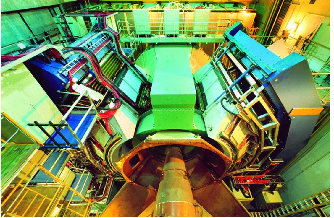
Figure 3.2: Photograph of the PHENIX detector viewed from north to south. The central arms are visible on the right (west) and east (left) sides. In the back the south muon magnet and the muon identifier detectors are visible.
