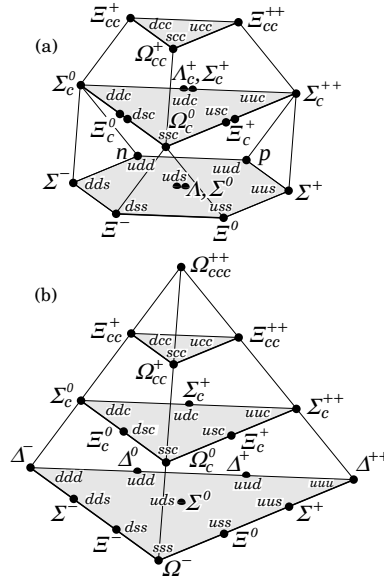
Figure 1.3: SU(4) multiplets of baryons made of u , d , s and c quarks. (a) The 20-plet with with a SU(3) octet. (b) The 20-plet with an SU(3) decuplet.
