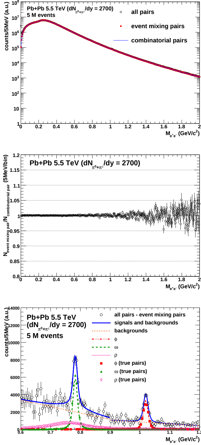
Figure 7.8: The invariant mass spectra in central Pb+Pb collisions at \sqrt{s_{NN}} = 5.5 TeV ( dN_{\pi^0+\pi^\pm}/dy = 2700 ) with the baseline experimental parameters: P_{cnn} = 1 %, R_{\pi^\pm} = 500 , \epsilon_{acc} = 100 %, \epsilon_{tag} = 100 %, p_T^{th} = 0.1 GeV/c and \sigma_{p_T}^{ref} = \sqrt{(0.01 \cdot p_T)^2 + (0.0056)^2} GeV/c.
