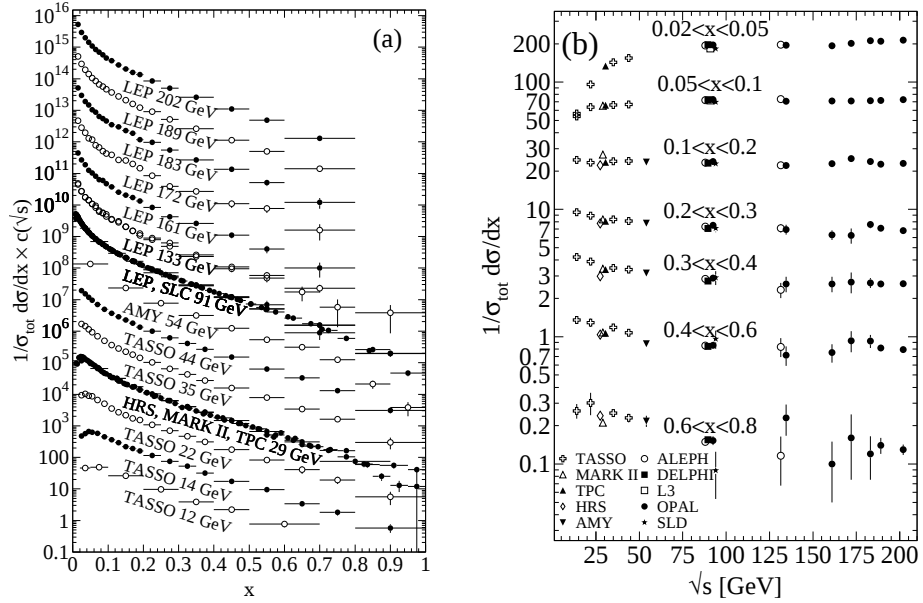
Figure 1.7: The fragmentation function in e^+e^- annihilation for all charged particles. (a) for different center-of-mass energy \sqrt{s} vs x scaled by c(\sqrt{s}) = 10^i with i ranging from i = 0 ( \sqrt{s} = 12 \text{ GeV} ) to i = 13 ( \sqrt{s} = 202 \text{ GeV} ) and (b) for various range of x vs \sqrt{s} .
