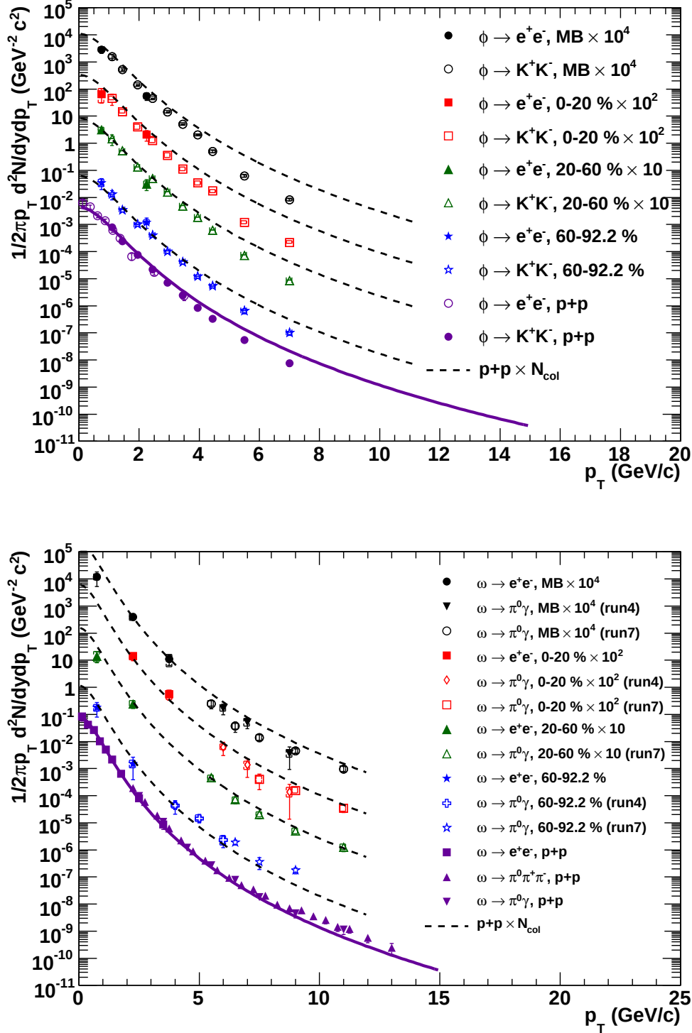
Figure 5.11: The comparison between the invariant transverse momentum spectra and the scaling curves via N_{\text{coll}} for \phi (top) and \omega meson (bottom). The scaling curves show the dotted lines. The shape of the curves are obtained from the fitting result to the p+p data [122] (solid line). The error bars and the brackets in the figure show the statistical errors and systematic errors, respectively. The data points of \phi \rightarrow K^+K^- and \omega \rightarrow \pi^0\gamma are cited from the references [132, 133].
