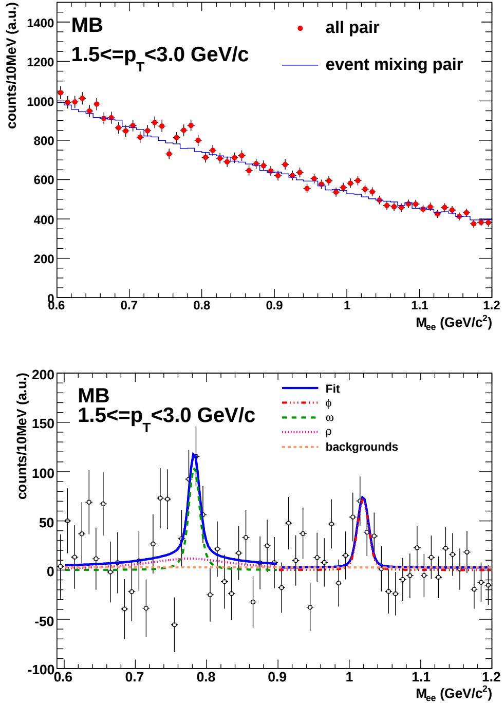
Figure 4.45: The invariant mass spectra of the di-electrons around the mass range of the light vector mesons (top). The invariant mass spectra of the di-electrons after subtracting the combinatorial backgrounds (bottom). The fitting results are superimposed in the plot.
