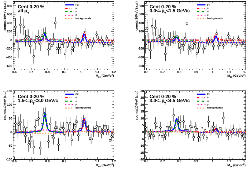
Figure 4.49: The invariant mass spectra of the di-electrons after subtracting the event mixing distribution at the centrality class of 0-20%
