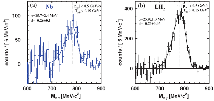
Figure 1.25: The invariant mass spectra of \pi^0\gamma momenta below 500 MeV/c and kinetic energy T_{\pi^0} > 150 \text{ MeV} for the Nb target ((a)), the \text{LH}_2 target ((b)) and Monte Carlo simulation [110]. The fitting curve takes into account the tail in the region of lower masses resulting from the energy response of the calorimeters.
